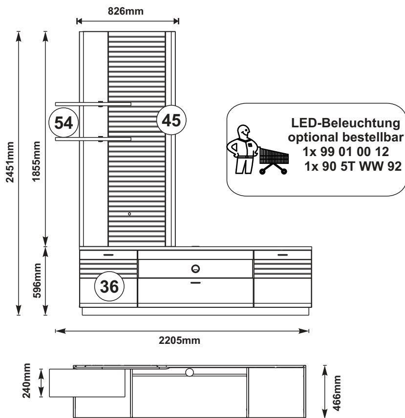
Kombination 40 C5 HW W2
