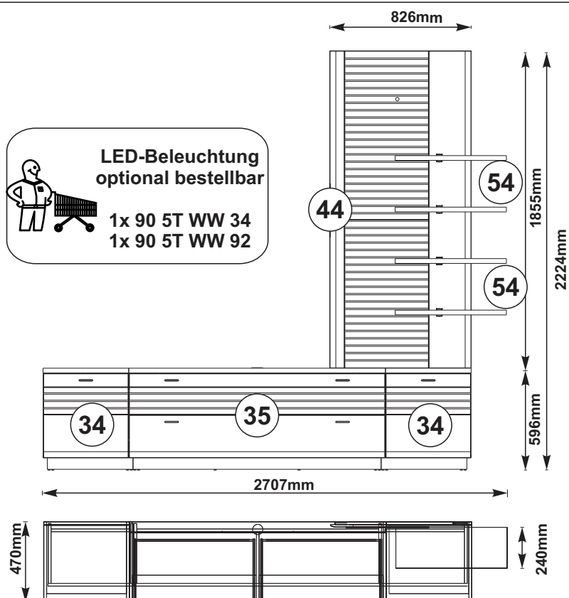
Kombination 40 C5HW U5
